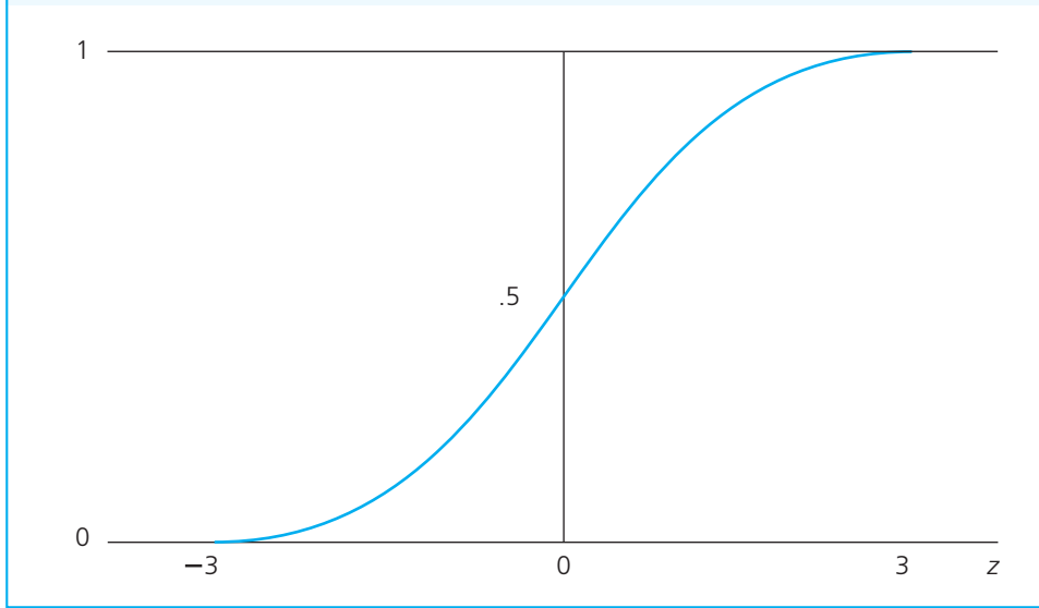
The standard normal cumulative distribution function.
