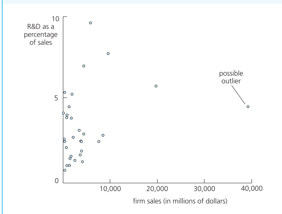
Scatterplot of R&amp;D intensity against firm sales.
